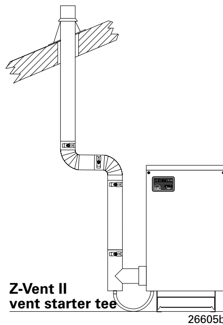
Figure 10 Non-direct vent through roof Follow Z-Vent II manufacturer's instructions for proper installation of vent runs, including slope and support.
