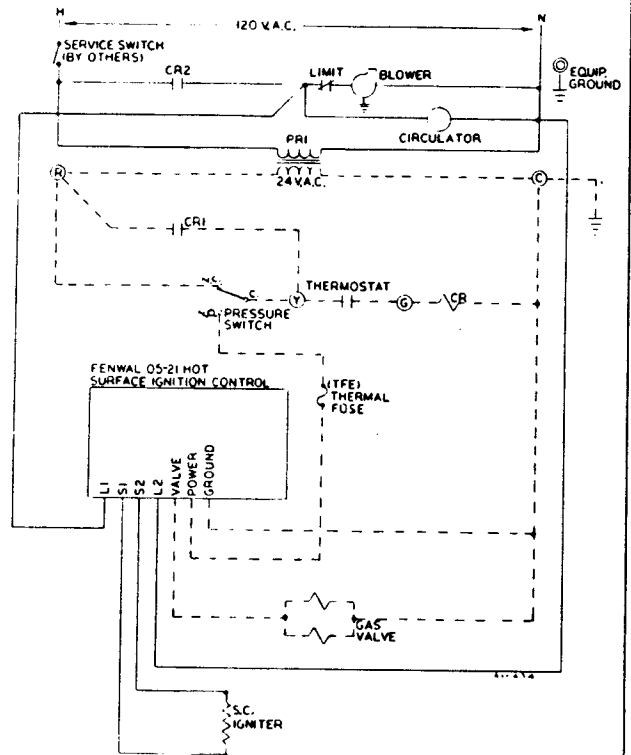
LADDER WIRING DIAGRAM
